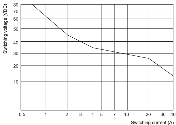
1. Load limit curve(at 25°C)
