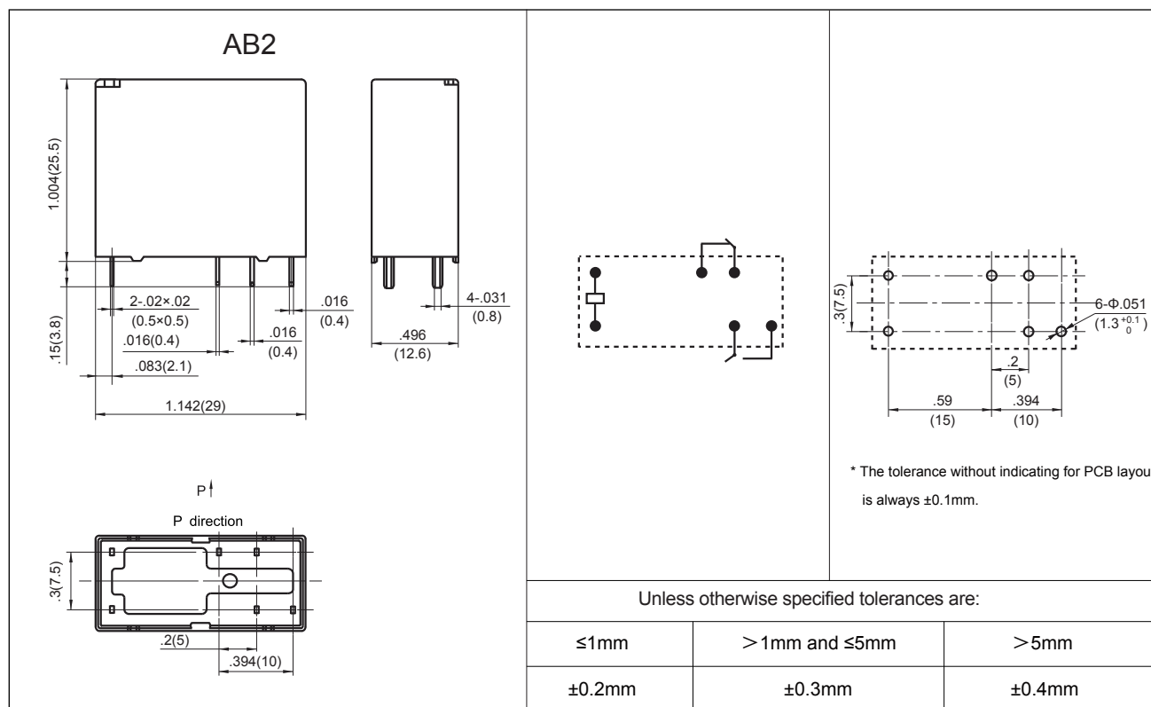
Wiring Diagram (Bottom view)
