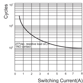
ELECTRICAL ENDURANCE
