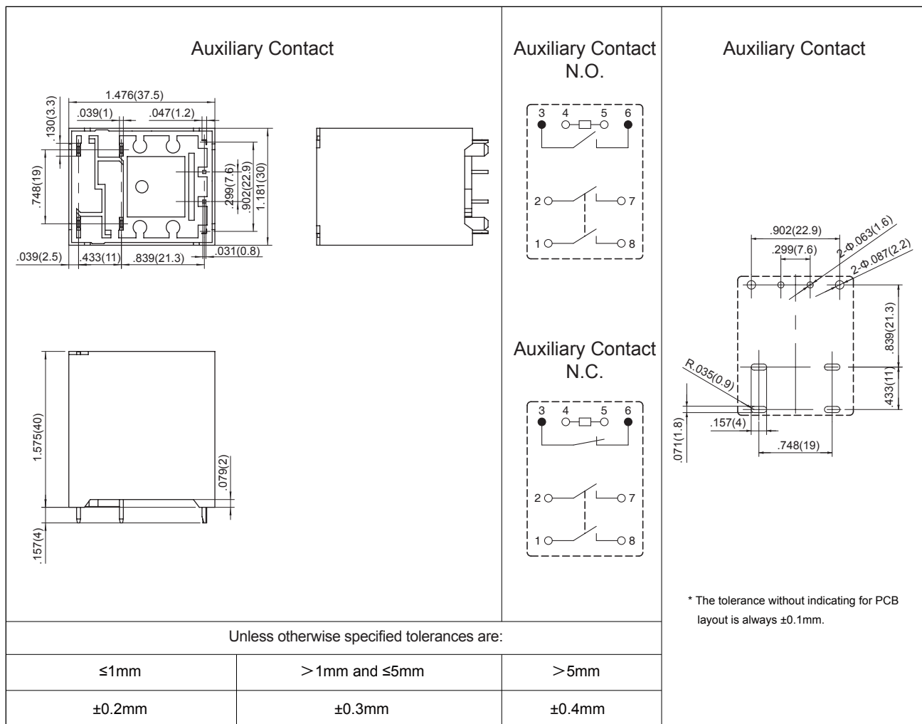
Wiring Diagram (Bottom view)
